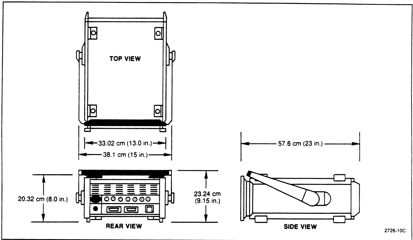
Figure 2-1. Dimensions.
